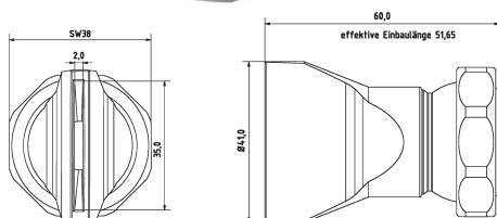
3-DU-SL-50-GS
