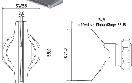
3-DU-SL-65-GS
