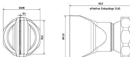
3-DU-SL-50-GS-0.4
