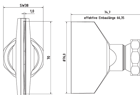
3-DU-SL-76-GS-0.4
