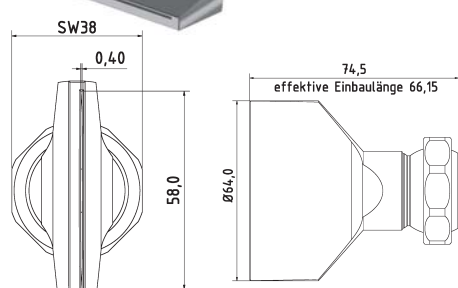
3-DU-SL-65-GS-0.4
