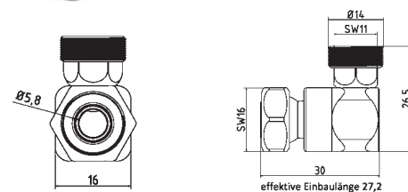
1-WV-1K Codo regulable
